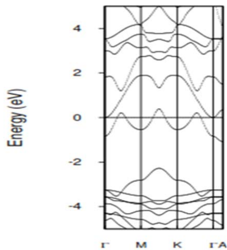
Fig. 14 Bands of WZ in Mg_{0.75}Bi_{0.25}O
