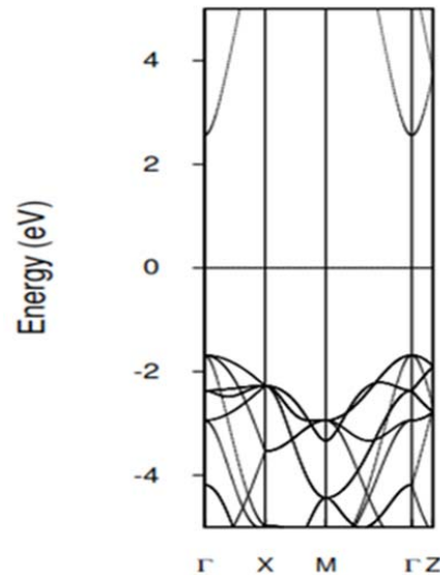
Fig. 9 Bands of NaCl in MgO
