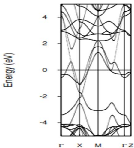
Fig. 12 Bands of NaCl in Mg_{0.25}Bi_{0.75}O
