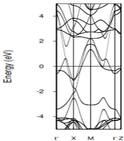
Fig. 11 Bands of NaCl in Mg_{0.5}Bi_{0.5}O
