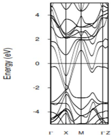
Fig. 10 Bands of NaCl in Mg_{0.75}Bi_{0.25}O
