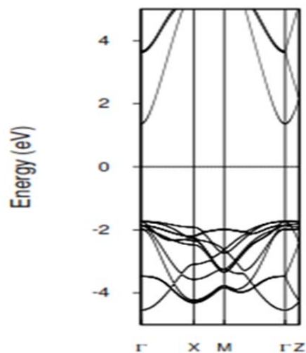
Fig. 13 Bands of WZ in MgO
