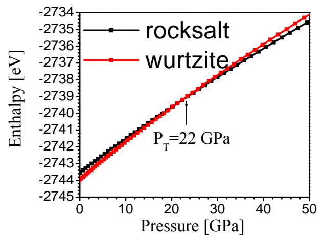
Fig. 6 Enthalpy vs. pressure
