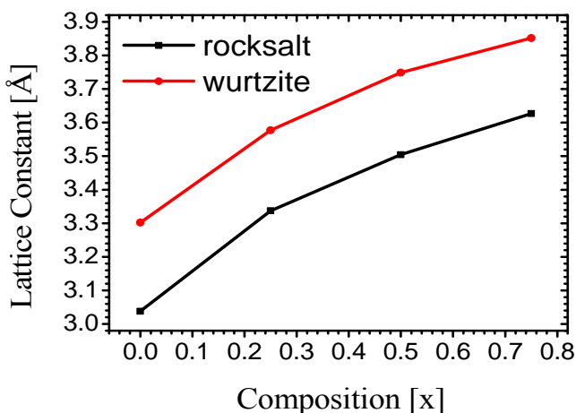
Fig. 7 Lattice constant vs concentration of Bi
