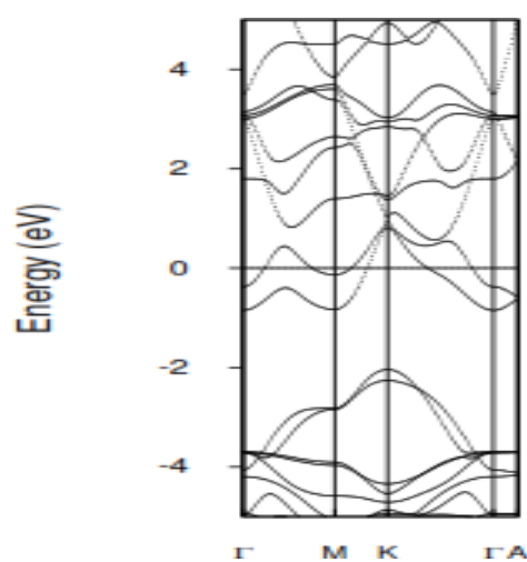
Fig. 15 Bands of WZ in Mg_{0.50}Bi_{0.50}O
