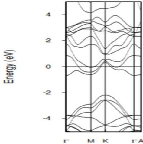
Fig. 16 Bands of WZ in Mg_{0.25}Bi_{0.75}O
