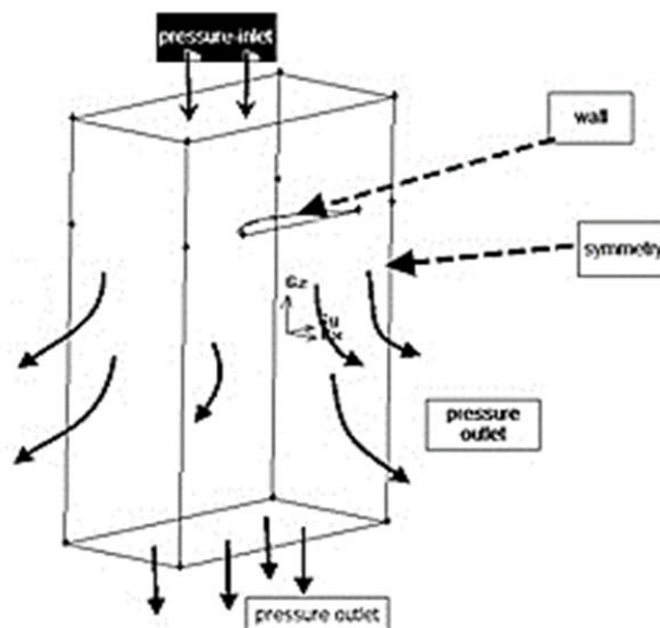
Fig. 2 Boundary conditions
