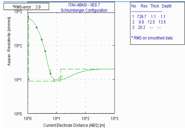
Fig. 7 Geoelectric Sounding Curve Obtained from VES 7
