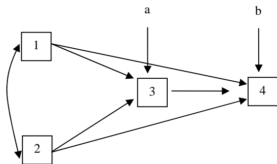
Fig. 1 An example of path analysis
