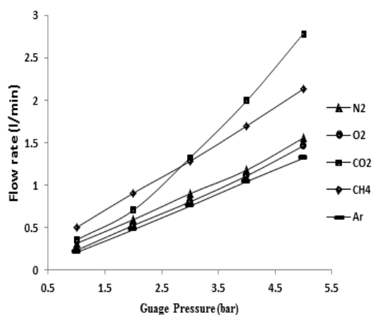
Fig. 4 Single gas flow rate measurement as a function of feed pressure at room temperature
