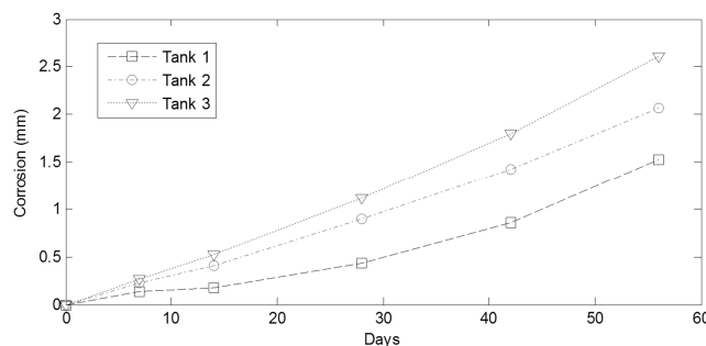
Fig. 4 Average corrosion depth of the cubes extracted at different days compared over three temperature regimes of sulphuric acid solution
