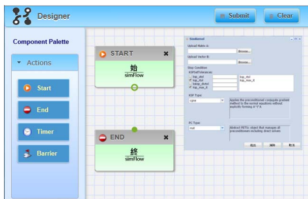
Fig. 3 Workflow Designer
