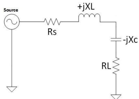
Fig. 1 A typical LC Matching Network
