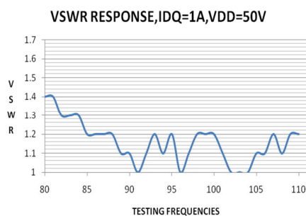
Fig. 7 VSWR Response
