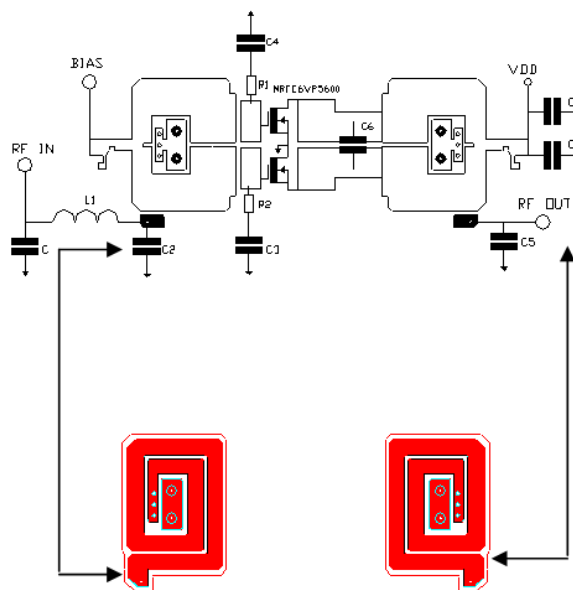
Fig. 6 Planar secondary
