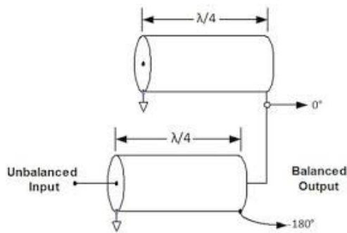
Fig. 3 Coaxial Type Balun
