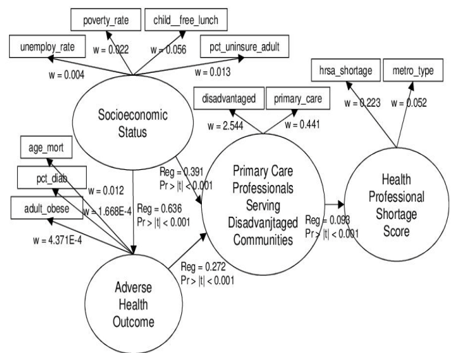
Fig. 2 PLS Path Model Diagram
