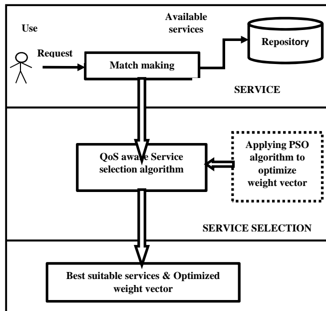
Fig. 1 Conceptual Architecture
