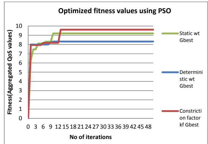
Fig. 3 Fitness analysis using optimized weight vector
