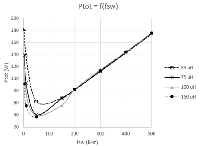
Fig. 8 Simulation results of SiC semiconductors power lost
