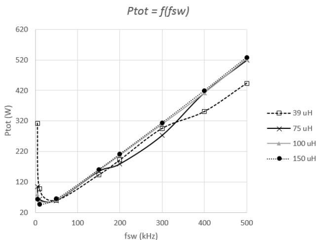
Fig. 12 Simulation results of Si semiconductors power lost
