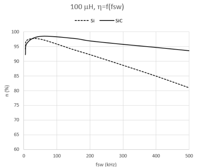
Fig. 14 Simulation results of Si and SiC converters efficiency for inductance 100 µH
