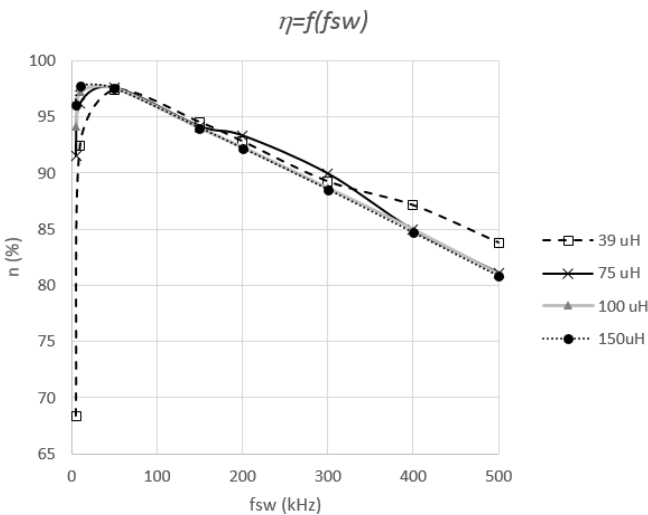
Fig. 11 Simulation results of Si converter efficiency
