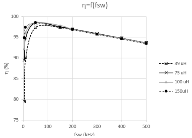
Fig. 7 Simulation results of SiC converter efficiency
