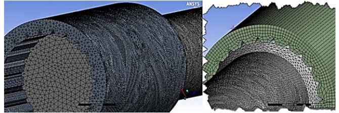
Fig. 3 3ds Meshed Model of axle of JD955 and JD1055 in ansys14 software
