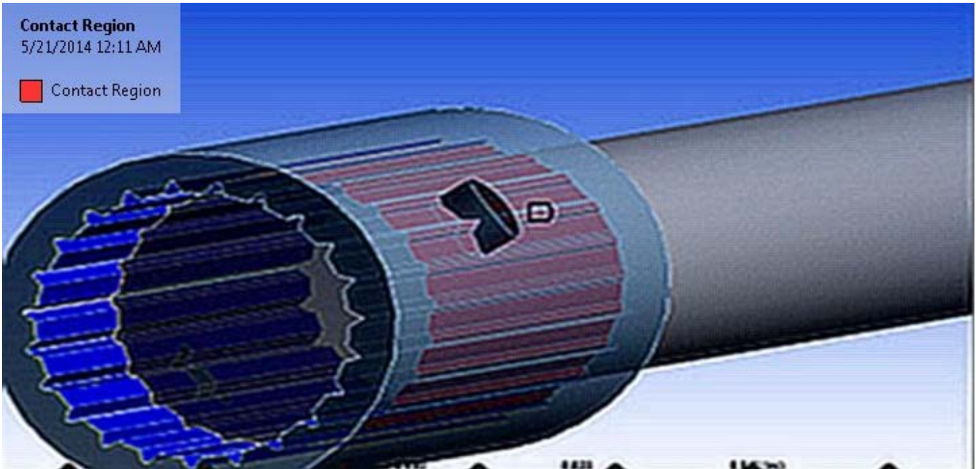
Fig. 4 Connection between Bushes in canal Combines JD955 & JD1055
