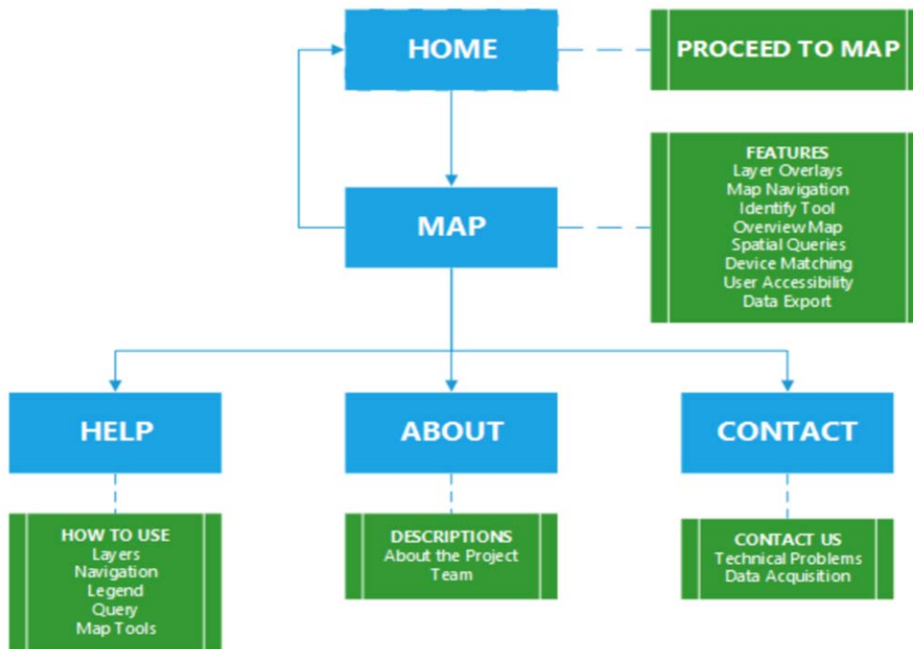
Fig. 4 Website section configuration
