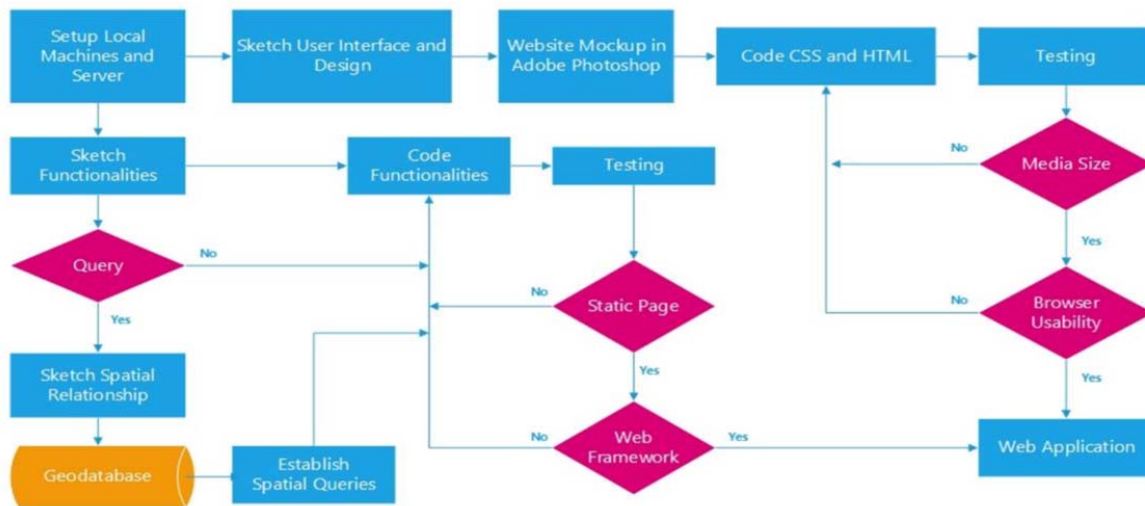
Fig. 2 Backend and frontend development workflow
