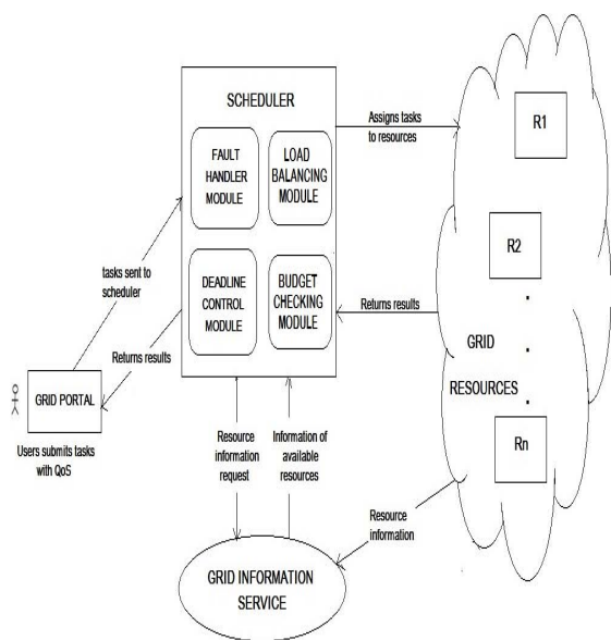
Fig. 2 BLBFT Architecture
