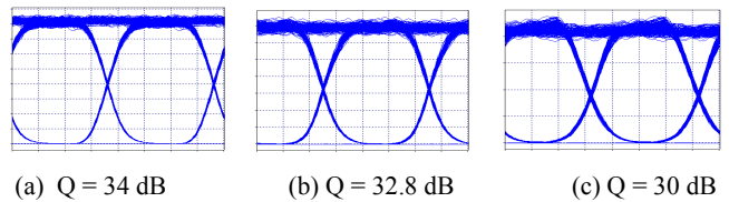
Fig. 17 Eye diagrams for signal input power of -15 dBm using six pump wavelengths, (a) single span (b) 5 spans (c) 10 spans
