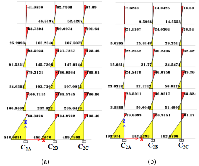
Fig. 7 Column bending moment distribution for two models (a) Bare frame (b) Masonry infill frame
