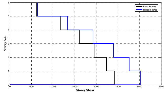
Fig. 4 Storey shear forces dynamic RS X-dir
