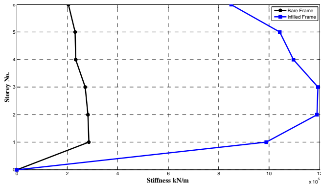
Fig. 3 Storey stiffness under dynamic RS X-dir
