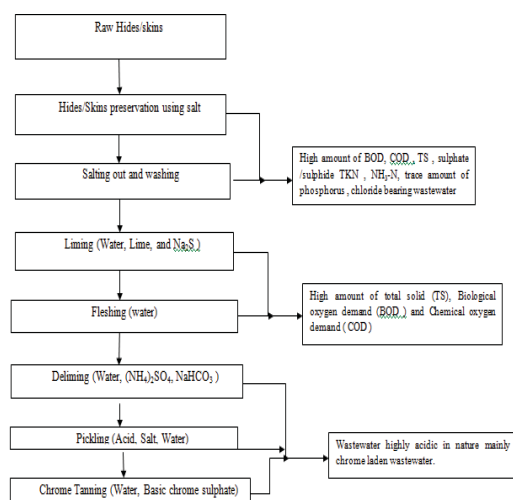
Fig. 1 Process Flow Diagram of a Typical Chrome Tannery unit
