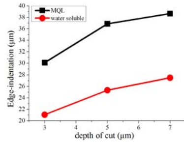
(a) V=565 m/min
