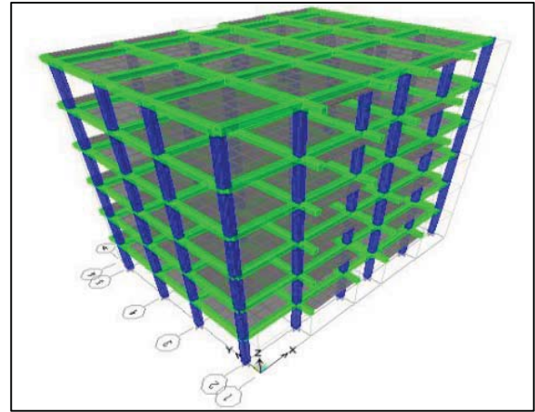
Fig. 4 3D view of the structure studied
