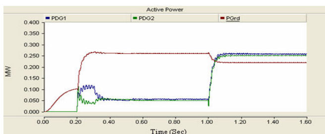
Fig. 8 Active output powers
