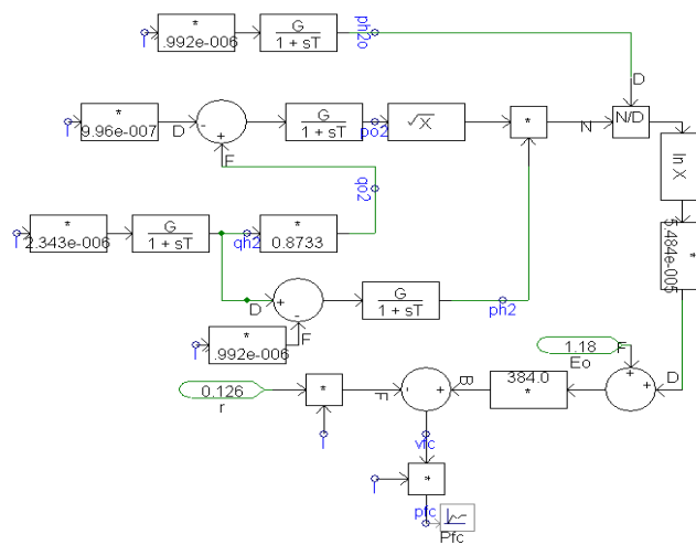
Fig. 4 PSCAD/EMTDC implementation of SOFC
