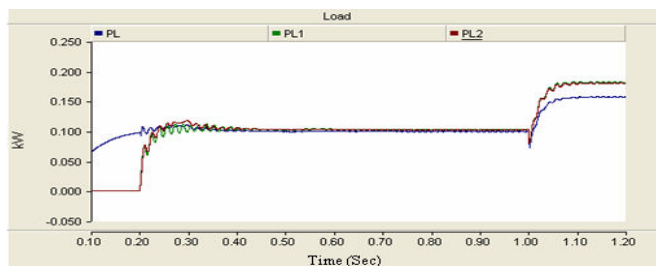
Fig. 9 Load powers
