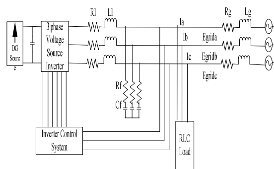
Fig. 3 Inverter control system for each distributed generation
