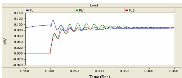
Fig. 11 Load powers
