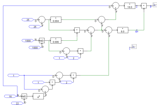
Fig. 5 PSCAD/EMTDC implementation of photovoltaic
