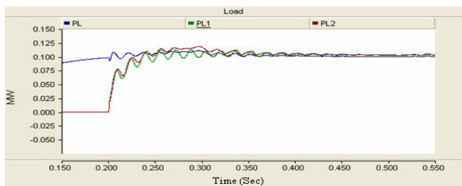
Fig. 7 Load powers
