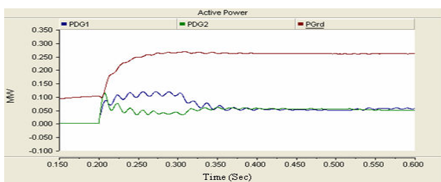
Fig. 6 Active output powers
