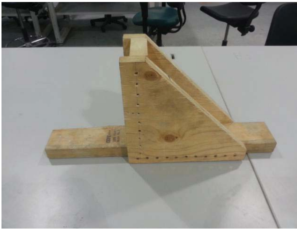
Fig. 1 The Shear Bond Test Apparatus
