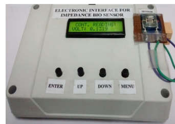
Fig. 7 Pictorial view of electronic interface
