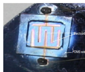
Fig. 3 Final view of the sensor
