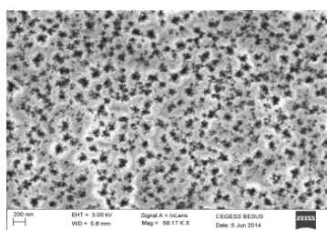
Fig. 2 (a) SEM image of oxidized nanoporous silicon
