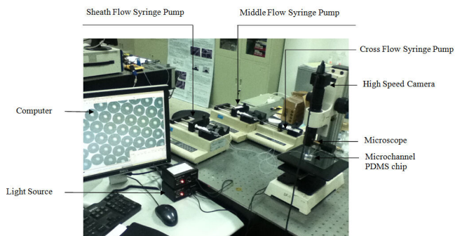
Fig. 4 Experimental set-up
