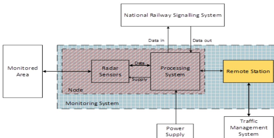
Fig. 1 System architecture
