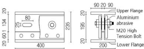
Fig. 9 Detail of shear friction damper [13]
