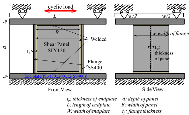
Fig. 3 Detail of Shear Panel Damper
