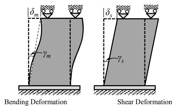
Fig. 7 Deformation mode of CHS damper
