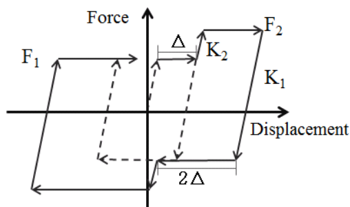
Fig. 11 The hysteresis response behavior of VRFD
