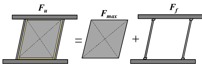
Fig. 4 Deformation mode of SPD
