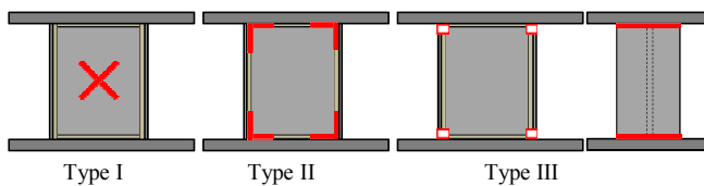
Fig. 5 Failure types of shear panel damper
