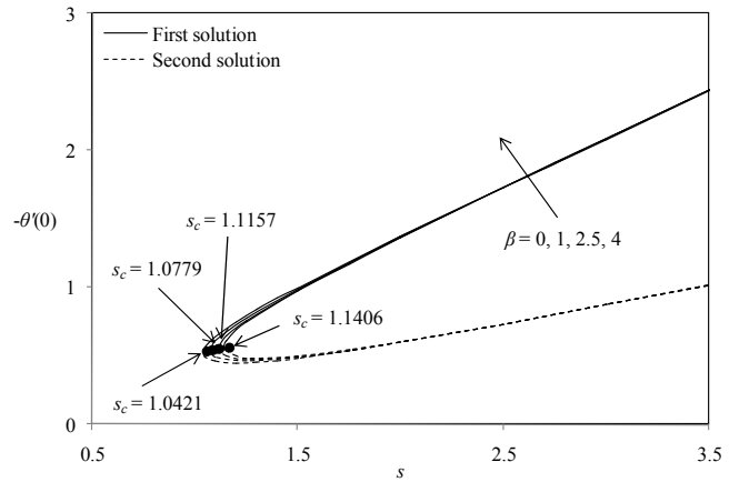
Fig. 4 Variation of -\theta'(0) with s for different \beta when \alpha = 5 , \lambda = -1 , Pr = 0.7
