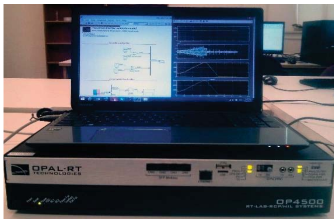
Fig. 14. OP4500, OPAL-RT real time simulator and RT-Lab software
