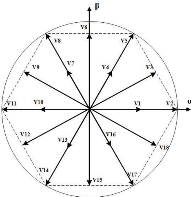
Fig. 3. Space voltage vectors of a three-level rectifier
