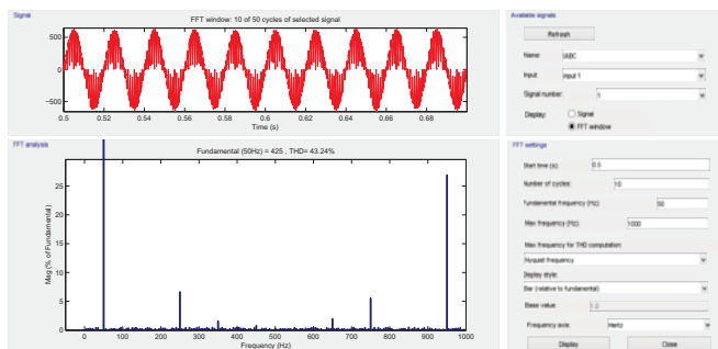
Fig. 12. The steady state source current and FFT analysis for DPC controller
