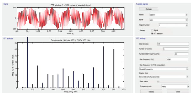
Fig. 13. The steady state source current and FFT analysis for conventional controller
