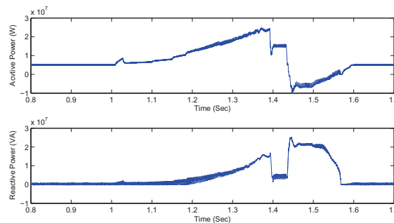
Fig. 11. Active and reactive power in DPC control
