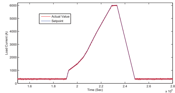
Fig. 15. Actual and reference value of load current using RTS
