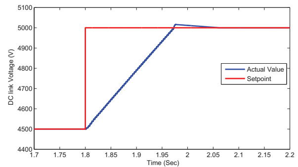
Fig. 5. Step response of DC link voltage
