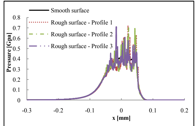
Fig. 6 Effect of surface roughness on pressure distributions with different kurtosis ( R_{ku} ) values
