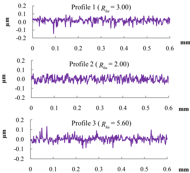
Fig. 1 Surface roughness profiles with different R_{ku}
