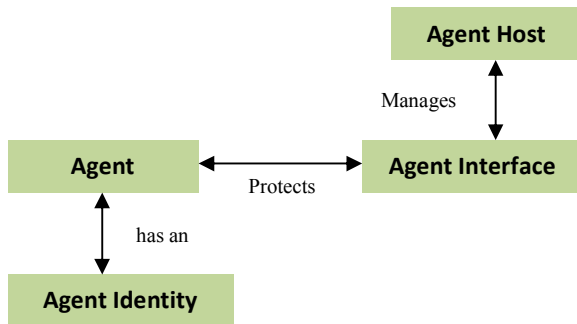
Fig. 1 Agent Architecture
