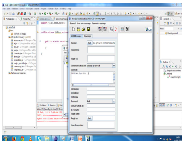
Fig. 5 Sending messages to other Agents
