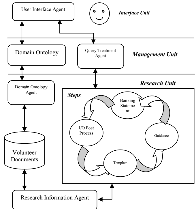
Fig. 2 System Architecture of Multi-Agent based Knowledge Acquisition
