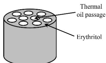
Fig. 3 Shell and tube thermal storage tank
