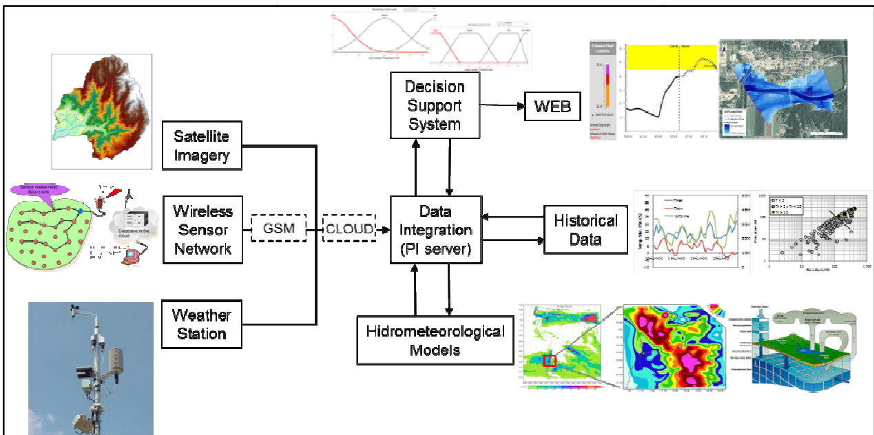
Fig. 6 Diagram of the pilot FFEWS for Quebrada de Ramón basin
