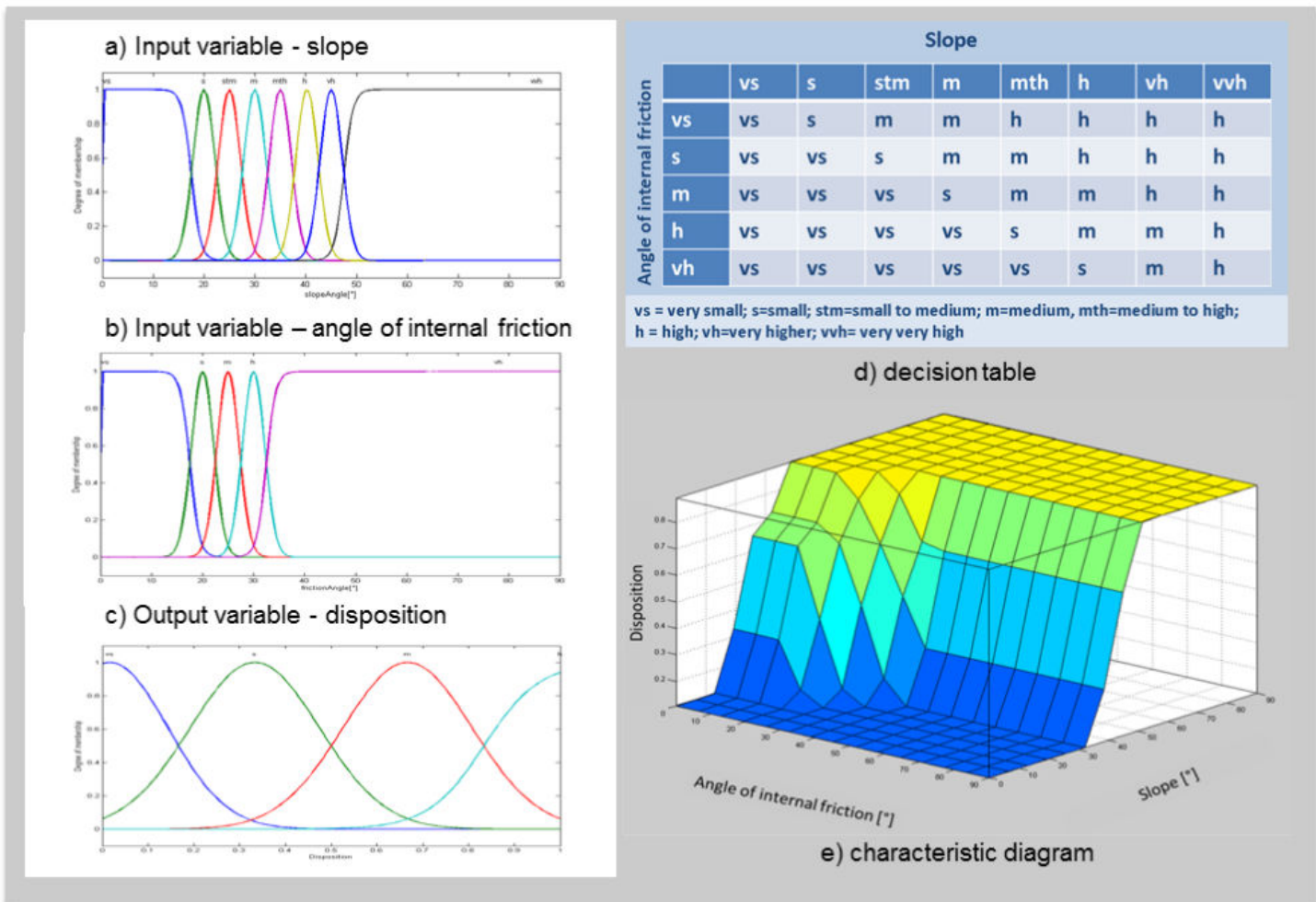
Fig. 5 Diagram of fuzzy expert systems from ELDEWAS [8]
