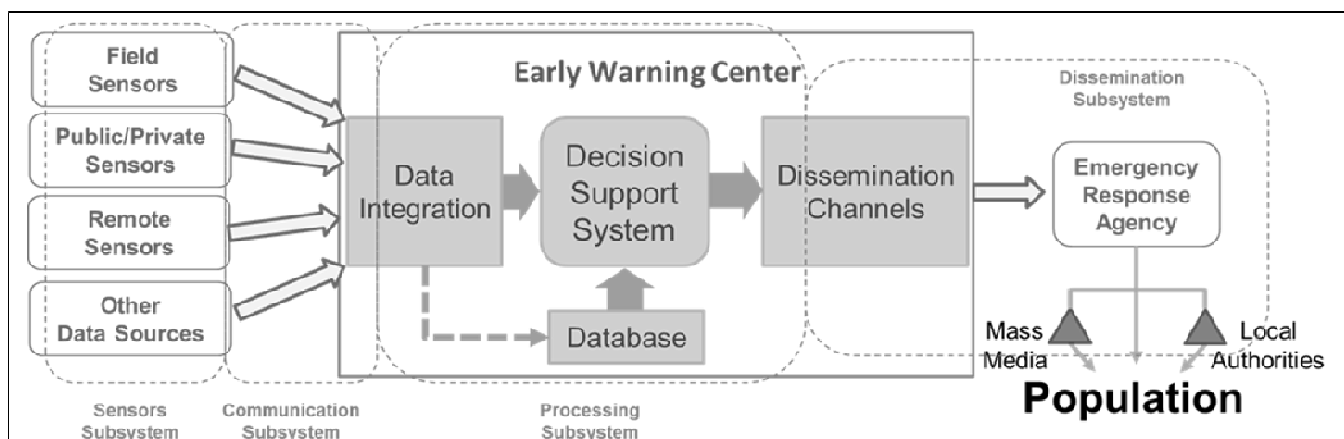
Fig. 3 Standard Early Warning System architecture
