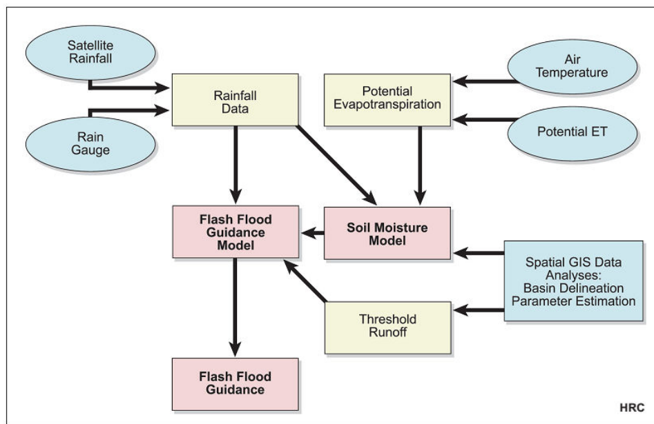
Fig. 1 Conceptual diagram of the CAFFG [5]
