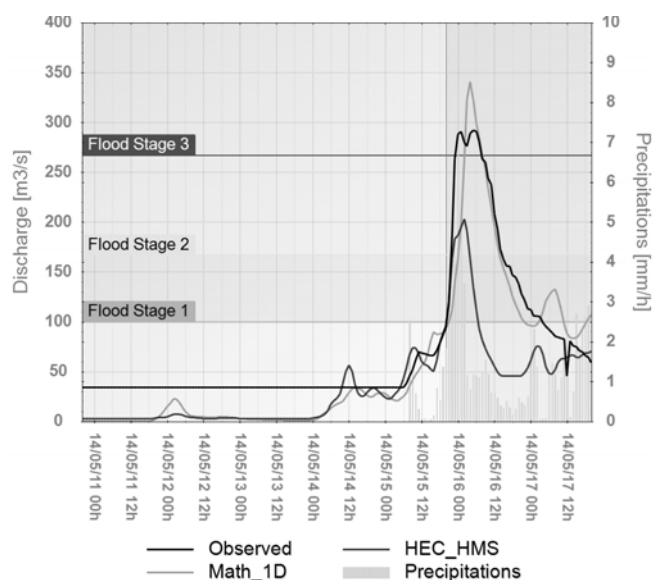
Fig. 2 Example of the rainfall-runoff model results
