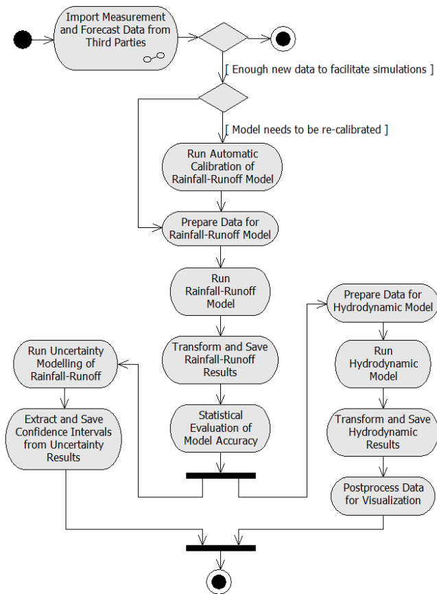
Fig. 1 Online flood prediction process
