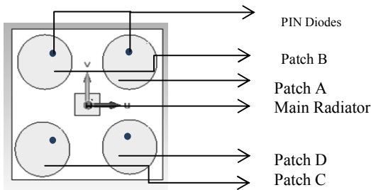
Fig. 3 Proposed antenna
