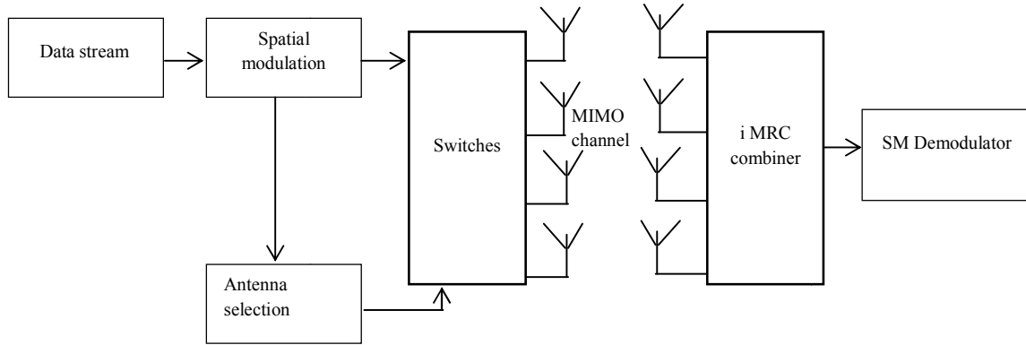
Fig. 1 Block diagram of conventional MIMO system
