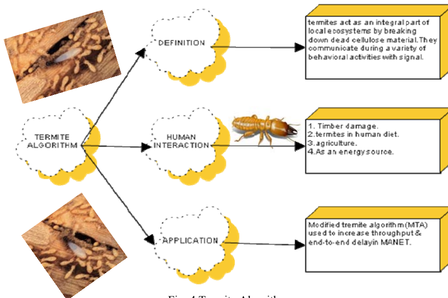
Fig. 4 Termite Algorithm
