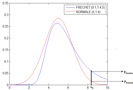
Fig. 4 Fréchet and normal distributions
