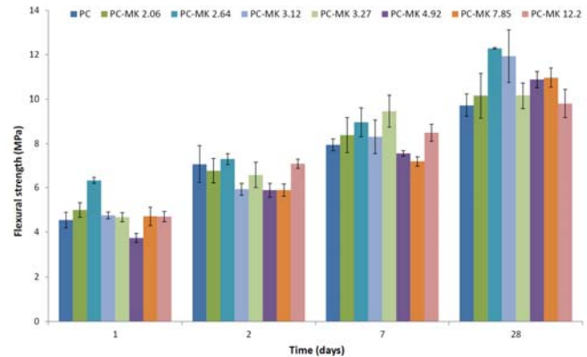
Fig. 3 The role of fineness of MK on flexural strengths development of samples
