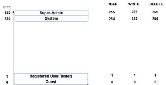
Fig. 1 Administrative authority roles with default Read, Write and Delete values
