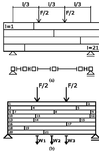
Fig. 6 (a) Model of laminated timber beam, (b) Actual location of all 21 segments in the examined beam
