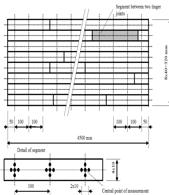
Fig. 2 Location of measuring points for the determination of local moduli of elasticity
