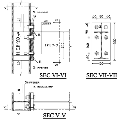
Fig. 3 Typical connection detail
