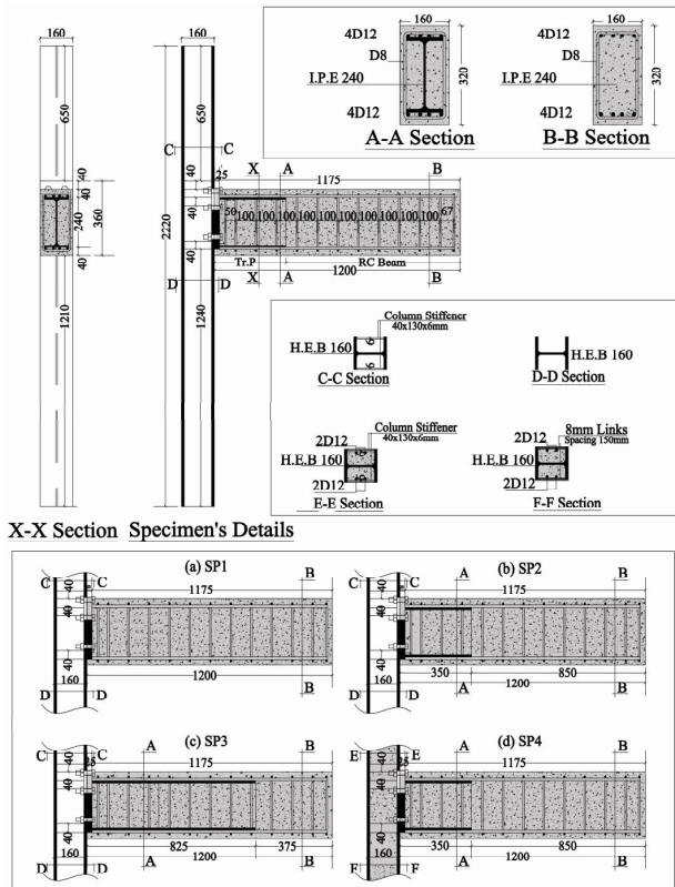
Fig. 2 All specimens details
