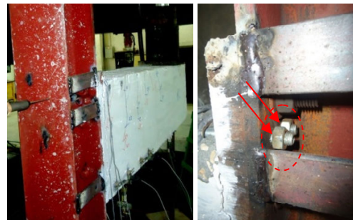
Fig. 12 Cracks in SP1 Beam and Splitting of the Steel Bars
