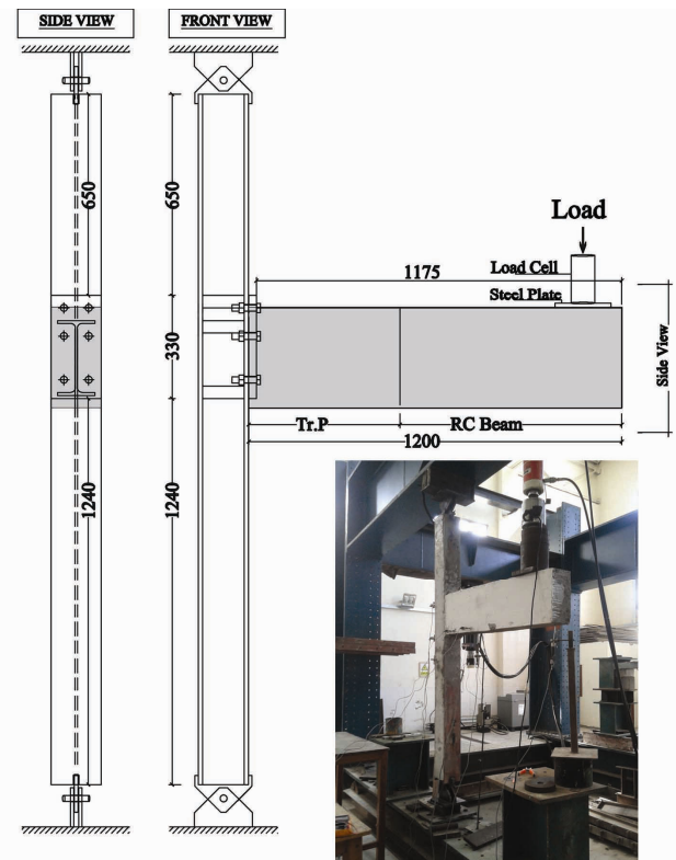
Fig. 4 Testing frame setup
