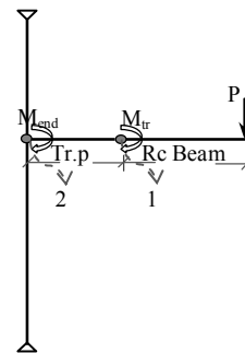
Fig. 9 Models static system
