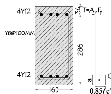
Fig. 10 Beams RC Section
