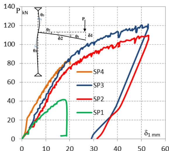
Fig. 5 Load-deflection relationship
