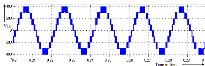
Fig. 16 Line to Line voltage of five level ZSI with simple boost technique
