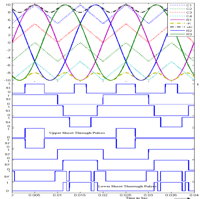
Fig. 8 Maximum constant Boost method with PD
