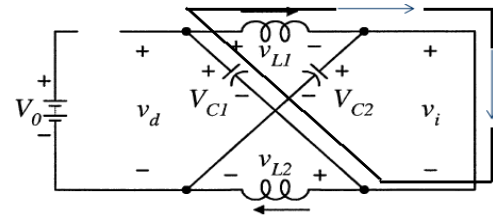
Fig. 5 Equivalent circuit in shoot through state
