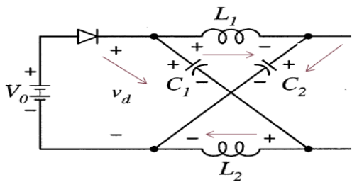
Fig. 3 ZSI Equivalent circuit in null states
