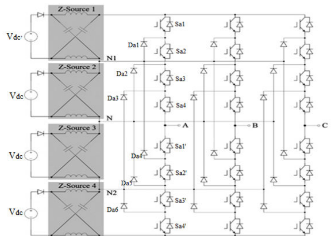
Fig. 6 Z source based five level Inverter
