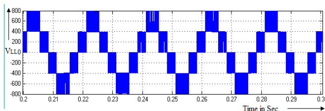
Fig. 13 Line to Line voltage of three level ZSI with simple boost technique
