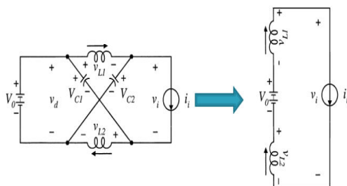
Fig. 4 Equivalent circuit in active states
