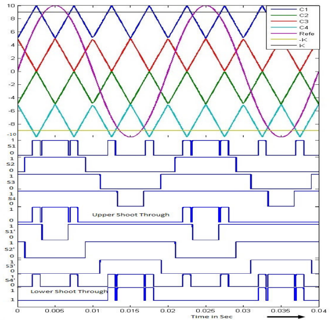
Fig. 7 Simple Boost Method with APOD
