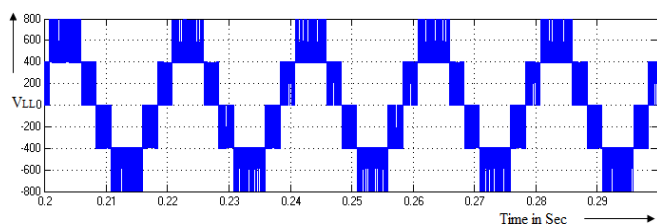
Fig. 14 Line to Line voltage of three level ZSI with maximum constant boost technique
