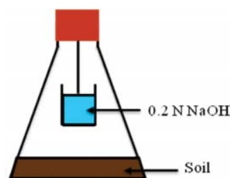
Fig. 3 Apparatus for measuring soil respiration rate
