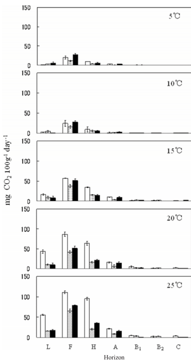
Fig. 4 Soil respiration rate at various temperature for laurel-leaved, C. japonica , and Hideyoshi C. japonica forest soils
