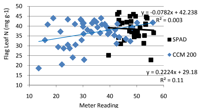
Fig. 4 Flag leaf nitrogen concentration versus meter readings
