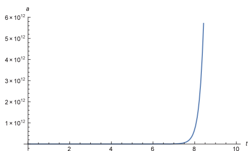
Fig. 1 The time dependence scale factor a .
