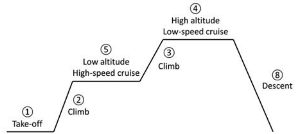
Fig. 4 Mission profile for case study
