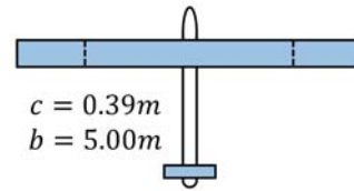
(a) Take-off configuration
