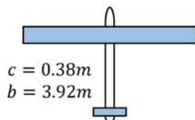
Fig. 5 Optimized fixed wing shape for the defined mission profile
