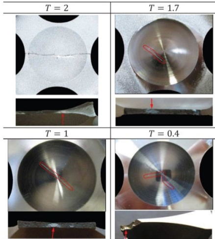
Fig. 7 Crack orientation within the cruciform specimen in respect to different stress state (triaxial stress ratio T) and macrographic observation of each rupture facies where crack propagation is clearly visible
