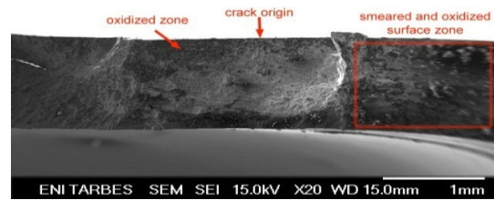
Fig. 10 SEM observation of a rupture facies in the case of a tension-compression test ( T=0.48 ). Smeared surface structures and oxidized zones (dark zones) are observed. Crack initiates from subsurface carbides and spread out elliptically through the thickness of the specimen
