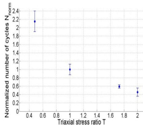
Fig. 6 Evolution of the normalized number of cycles to crack initiation with respect to the triaxial stress ratio. Mean points) and standard deviation (error bars) are plotted
