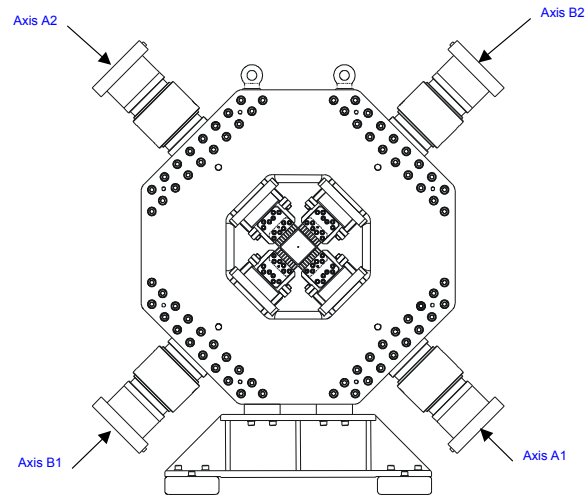
Fig. 3 Visualization of the biaxial testing machine
