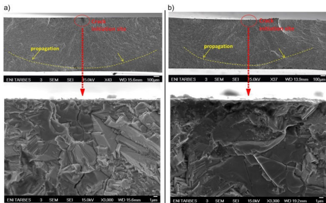
Fig. 8 SEM observations of crack propagation and cracked carbides on rupture facies of cruciform specimens under in-plane biaxial cyclic loading. a) proportional equibiaxial tension-tension test at 95 kN; b) proportional tension-tension test at 60 kN / 89 kN
