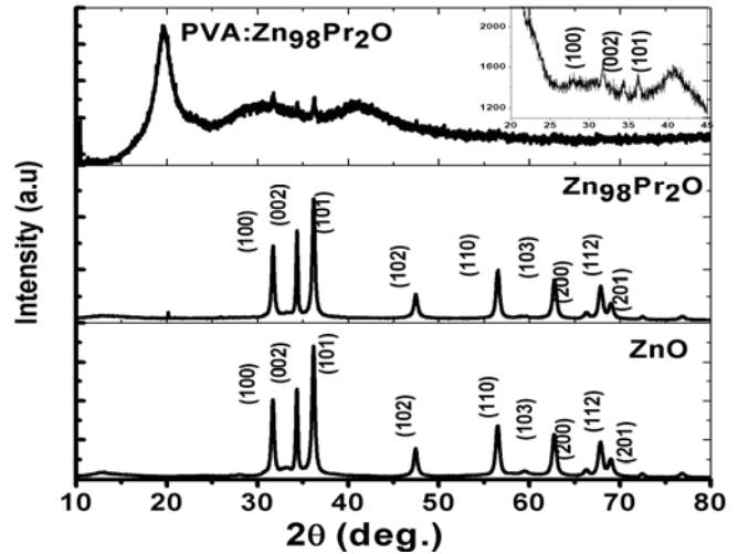
Fig. 1 XRD spectra of pure ZnO, Pr doped ZnO nanostructures and PVA: \text{Zn}_{98}\text{Pr}_2\text{O} polymer nanocomposite free standing film
