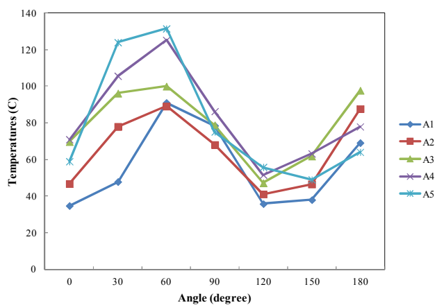
Fig. 8 The relationship between temperature distribution and the rotation angle of NRG at various positions
