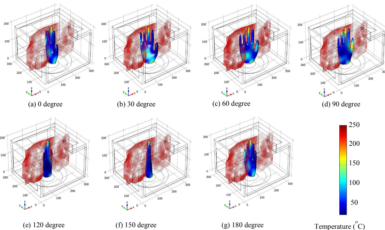
Fig. 6 The electric field and temperature distribution in NRG during microwave heating based on P = 100\text{ W} and t = 180\text{ s} at various rotation angle of NRG
