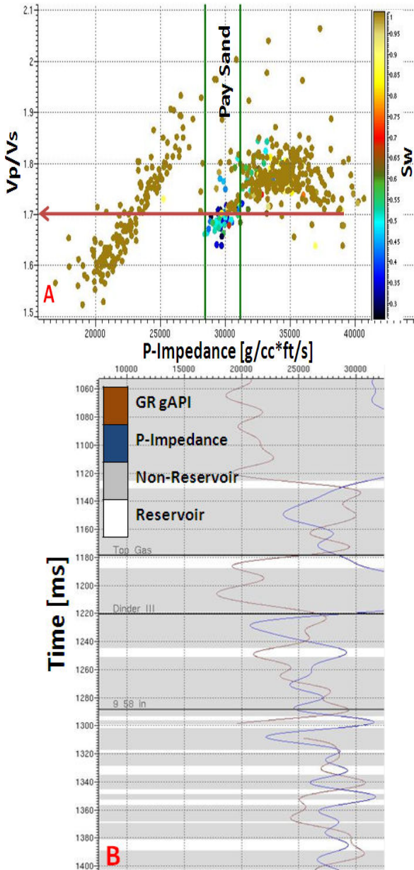
Fig. 4 (A) P-impedance versus V_p/V_s in water saturation color scale in HSN-1. Crossplot interval from 1460-1600 m. The Pay sand could be isolated in log resolution by using range values (green lines) in P-impedance axes, and also it can be confirmed by using the value (1.7 and below) as a cutoff from V_p/V_s (B) the corresponding well log
