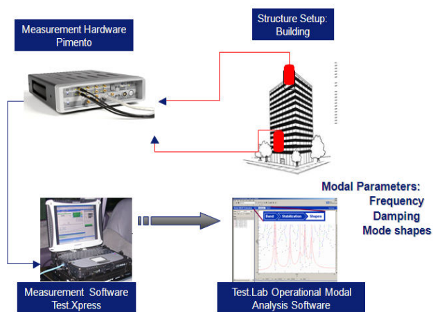
Fig. 3 Measurement system
