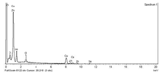
Fig. 3 (b) EDS spectra of annealed ZnSe film
