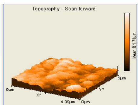
Fig. 4 (b) AFM photographs of annealed ZnSe
