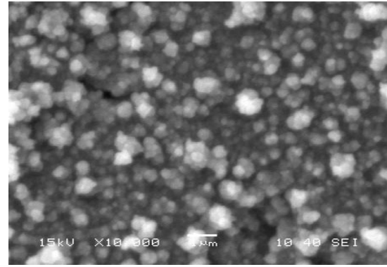
Fig. 2 (a) SEM photograph of annealed ZnSe film
