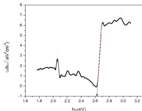
Fig. 5 (b) (\alpha hv)^2 vs hv spectra of annealed ZnSe film
