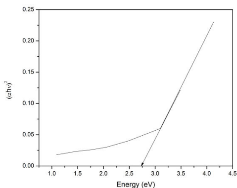
Fig. 5 (a) (\alpha hv)^2 vs hv spectra of as deposited ZnSe film
