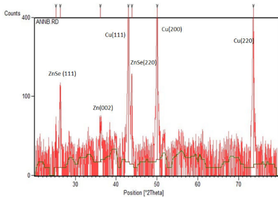
Fig. 1 (b) XRD Spectra of annealed ZnSe film
